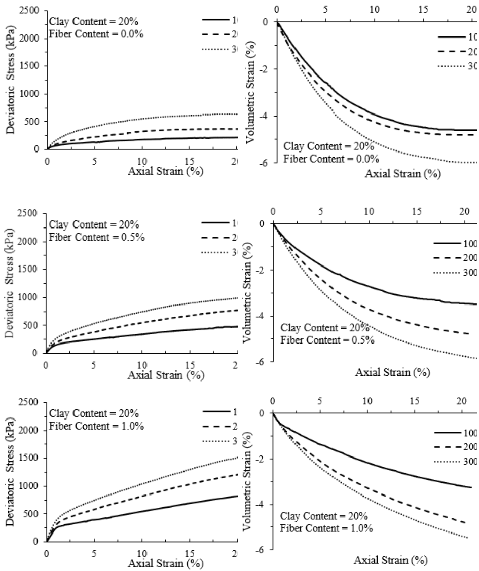
Figure 4. Deviatoric stress-axial strain (on the left) and volumetric strain-axial strain curves (on the right) of unreinforced and fiber-reinforced samples with D_r = 50\% and clay content = 20%
