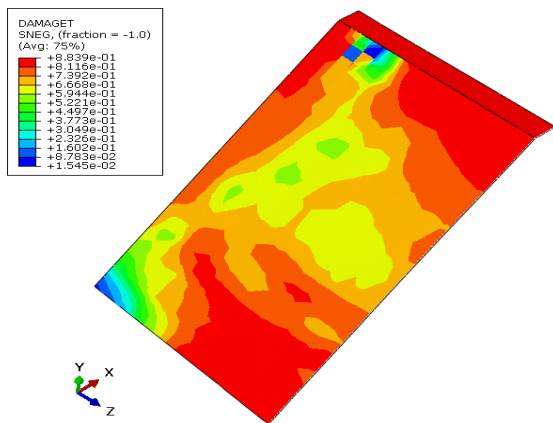
Step: Step-1 Increment: 18204; Step Time = 17.20 Primary Var: DAMAGE Deformed Var: U; Deformation Scale Factor: +1.000e+00
