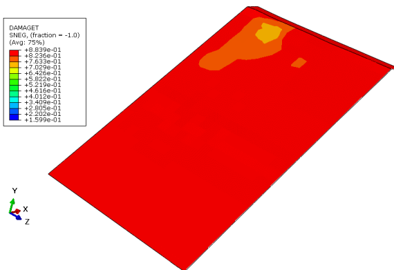
Step: Step-1 Increment: 18333; Step Time = 17.20 Primary Var: DAMAGE Deformed Var: U; Deformation Scale Factor: +1.000e+00
