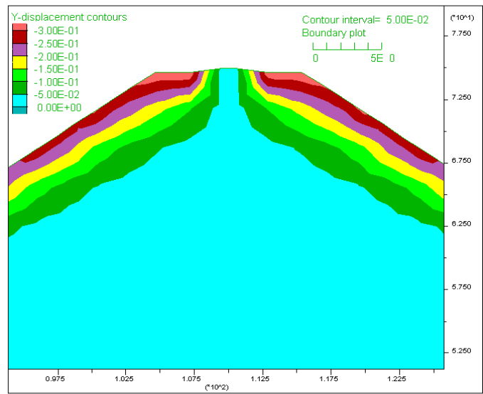
Fig.9. Settlement contours in dam crest area
