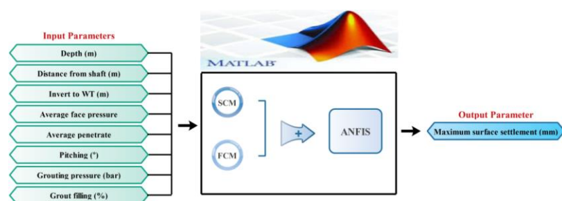
Figure 4. Architecture of the ANFIS based on the SCM and FCM.
