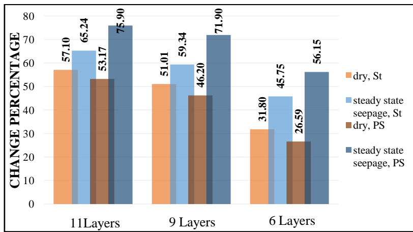
Figure 13. Horizontal displacement variations in horizontal layered models
