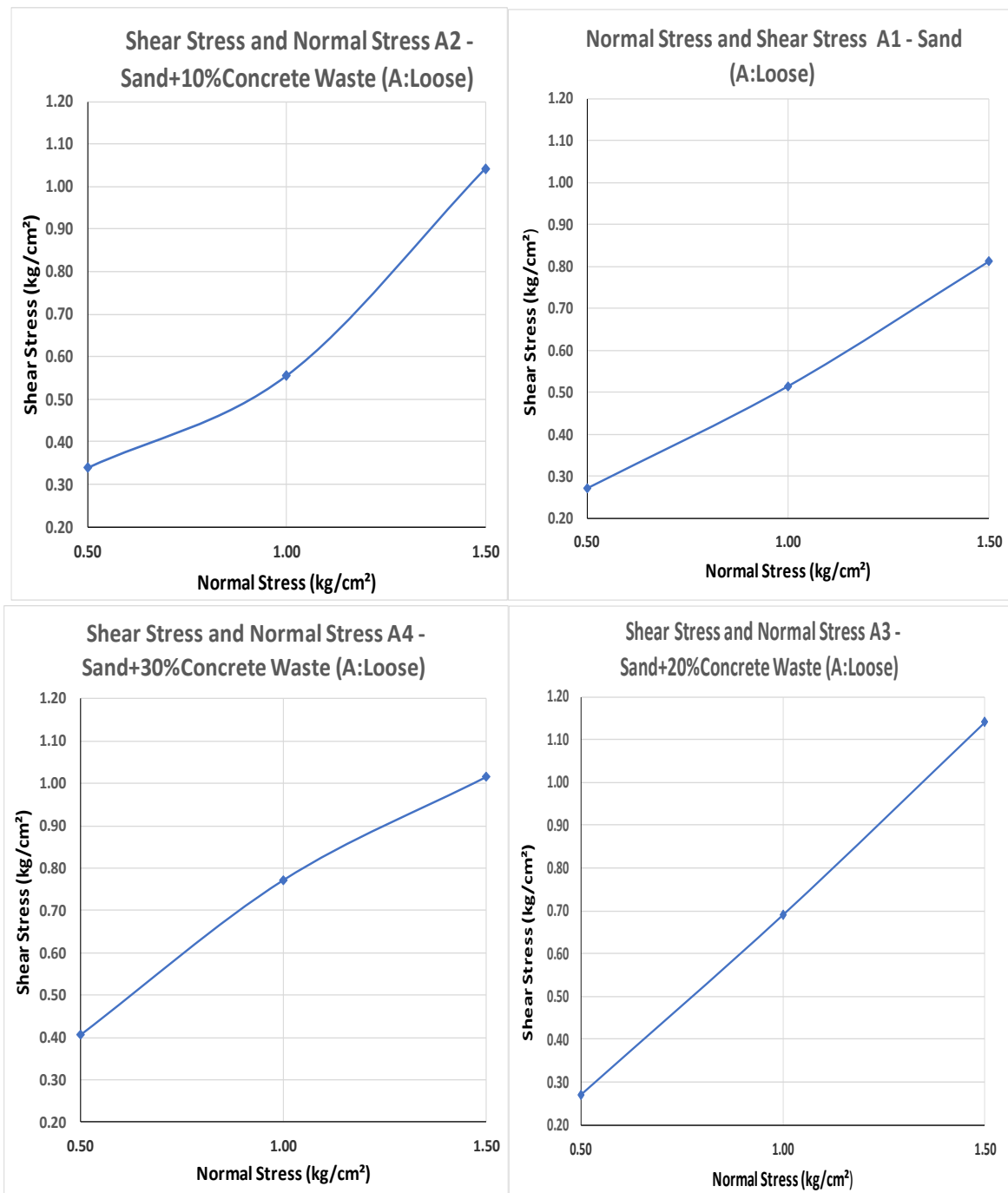
Fig. 2. Shear Stress - Normal Stress diagram for loose sand (samples A)
