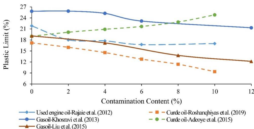
Fig. 13. CL soil plastic limit by type of contamination
