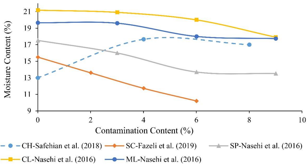
Fig. 4. Optimal moisture percentage of soil contaminated with gas oil
