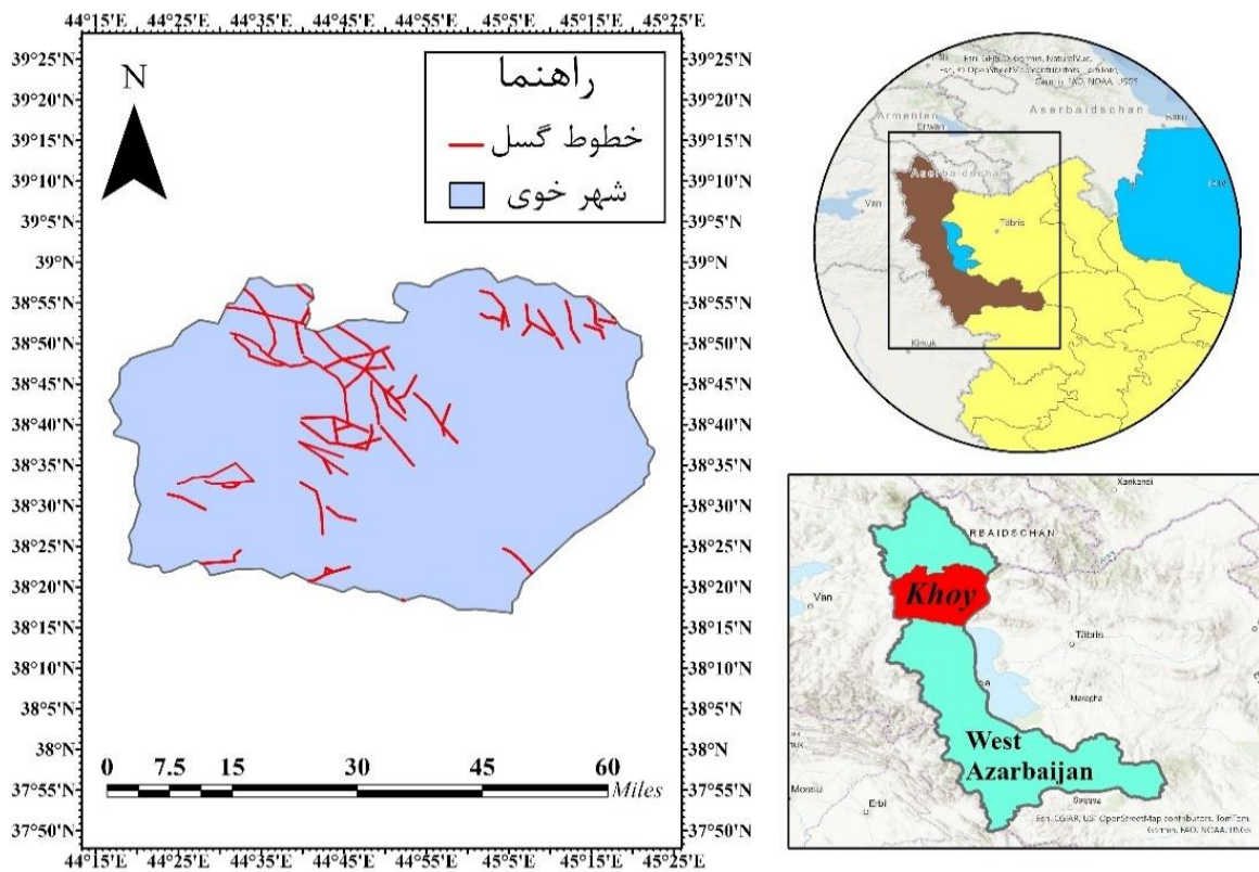
Fig. 1. Displaying the study area boundaries and the map of its fault lines
