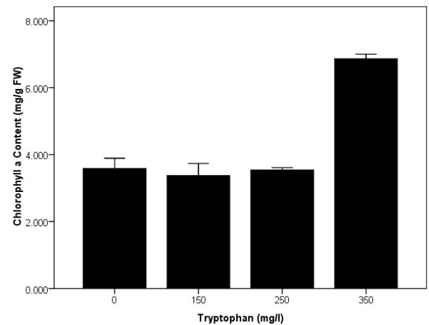
Figure1. Effect of tryptophan on chlorophyll a content of C. roseus . Results are shown as mean \pm standard error ( P < 0.05 ), obtained from four replicates
