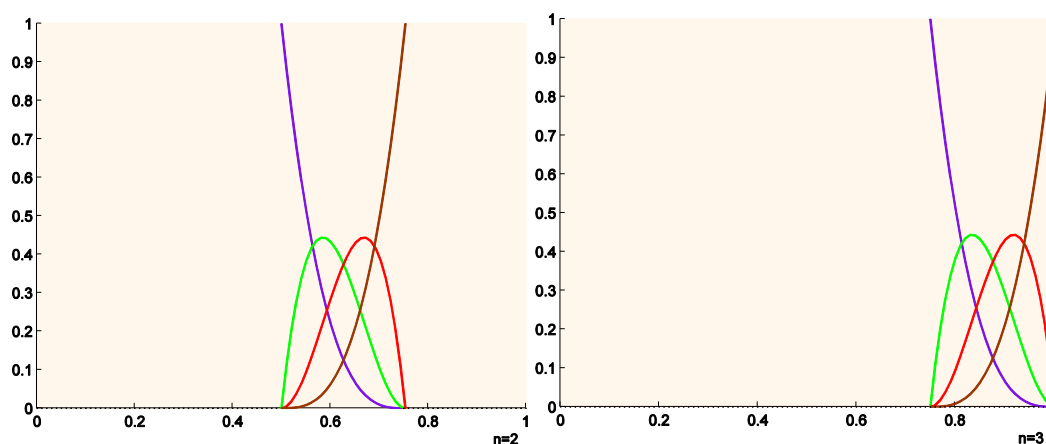
Figure 1: Graph of BMS functions for (m = 3; k = 4)
