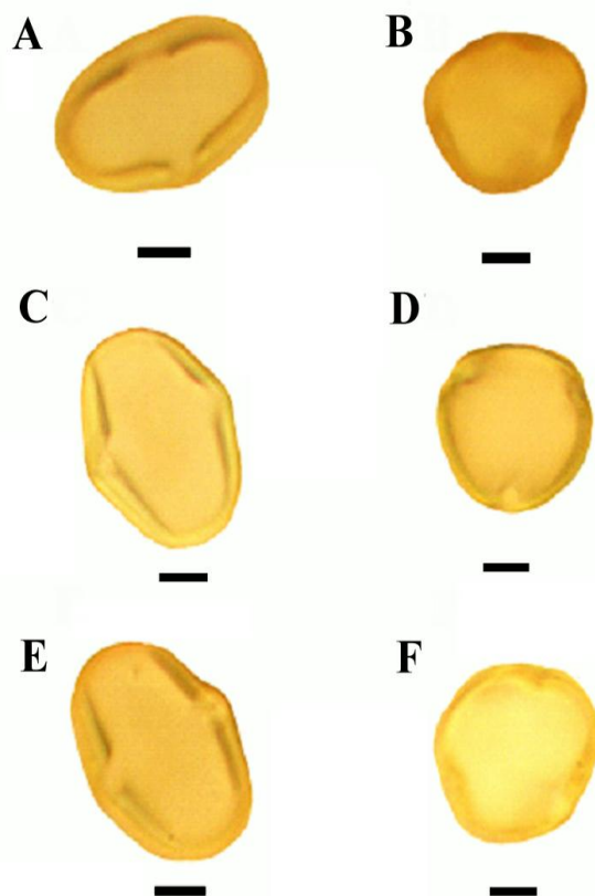
Fig. 4. LM polar and equatorial views of the pollen grains in three Trigonella species: A, B: T. aphanoneura ; C, D: T. disperma ; E, F: T. subnervis . Scale bars = 6 µm.
