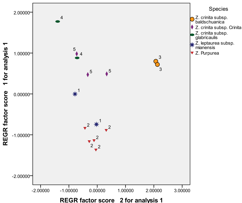
Fig. 9. PCA of the first and second factors based on Morphological quantitative cypselas features.
